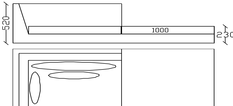
3 seater short back art. no. 77.03 LEFT art. no. 77.13 RIGHT
