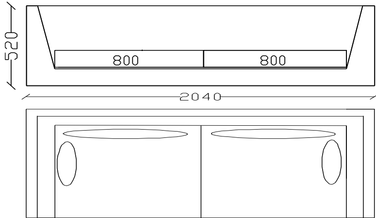
2,5 seater art. no. 77.05
