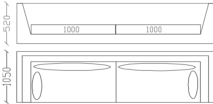
3 seater art. no. 77.01
