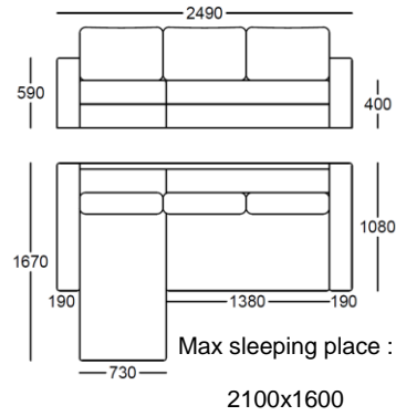
Corner group Left
