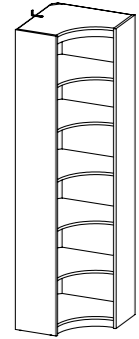
65016 Inside bookcase corner for 65012, 65013 60.3 x 60.3 x 213.9 cm 23.7 x 23.7 x 84.2" Colour: 18
