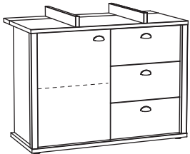
BKO 120 x 96 (88) x 66 (51) cm
