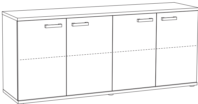
DR20 200 x 85 x 50 cm
