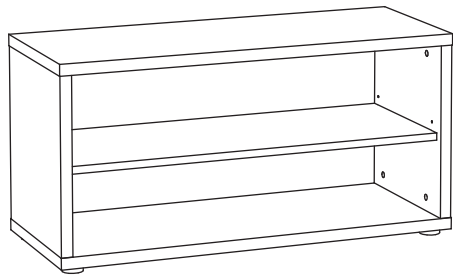
TV 100 x 50 x 40 cm
