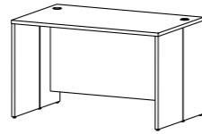
81202 Desk 120.9 x 75 x 73.4 cm 47.6 x 29.5 x 28.9" Colours: 20
