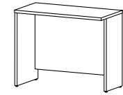
81215 Desk extension, reversible 92.4 x 44.5 x 73.4 cm 36.4 x 17.5 x 28.9" Colours: 20 - 33
